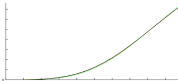
FIGURE 2. Relation of B and error for example 6.1 for \alpha = 1.1 , \beta = 1 , \sigma = 0.2 , m = 3 , k = 2
